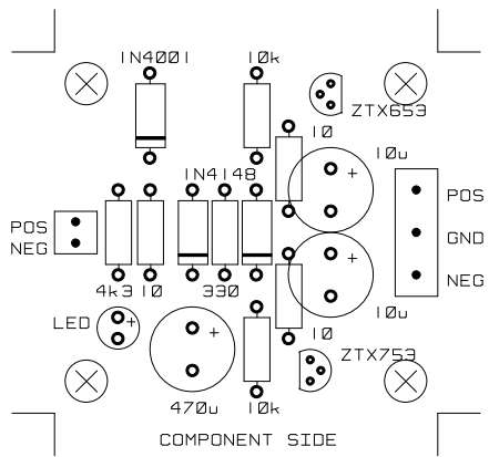
DC SPLITTER V1.0
